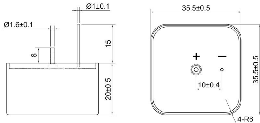
Dimensions: 35.5x35.5x20mm
