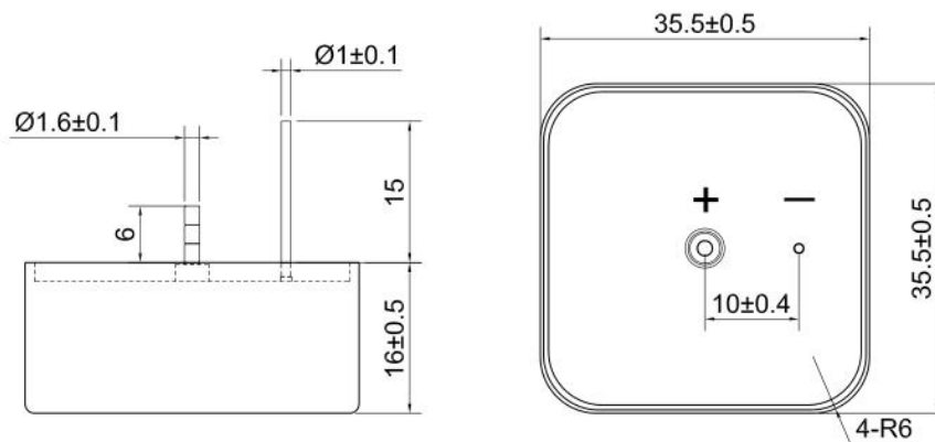
Dimensions: 35.5x35.5x16mm
