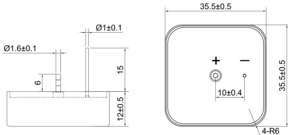
Dimensions: 35.5x35.5x12mm
